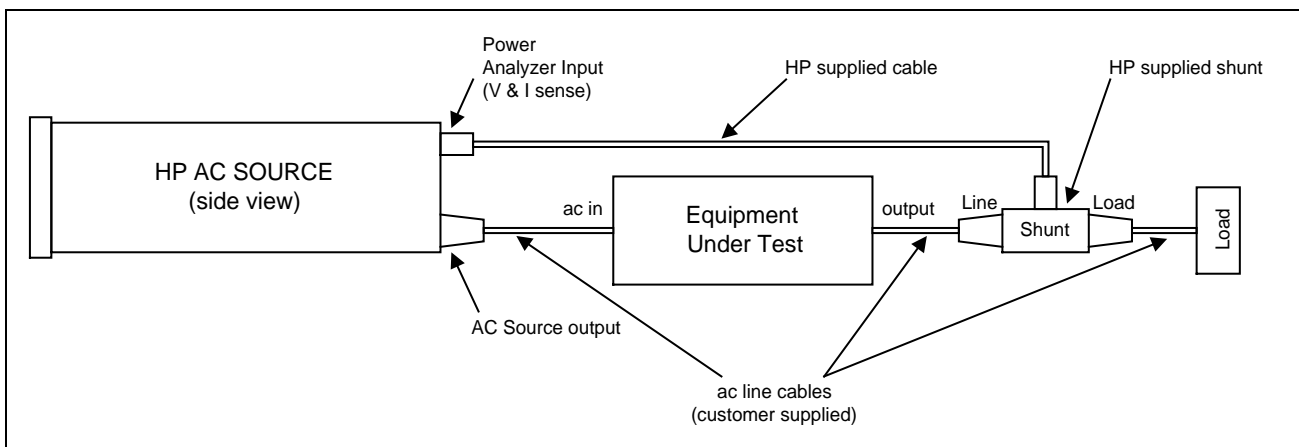
Option 020 Typical Connections
