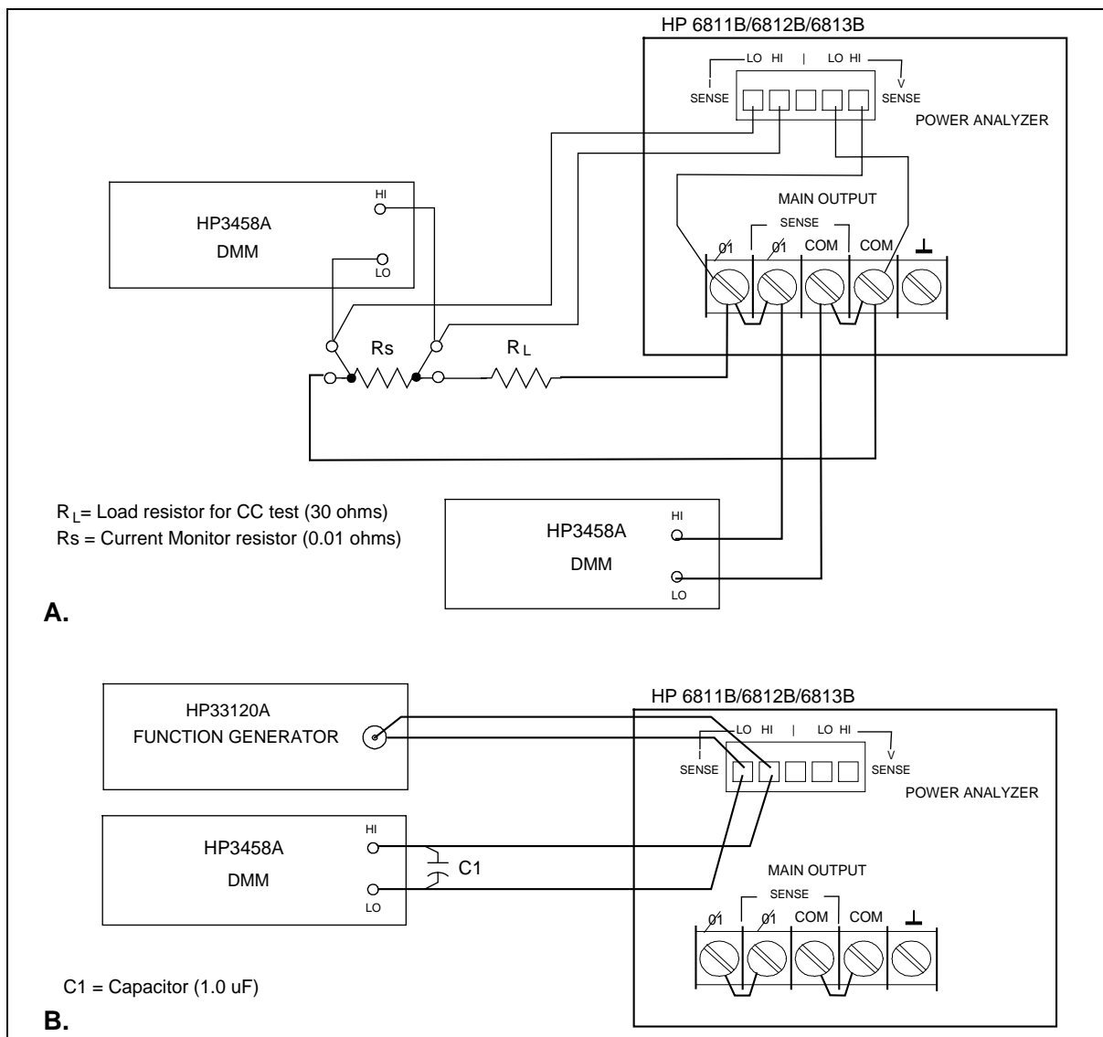
Figure B-1. Verification / Calibration Test Setup
